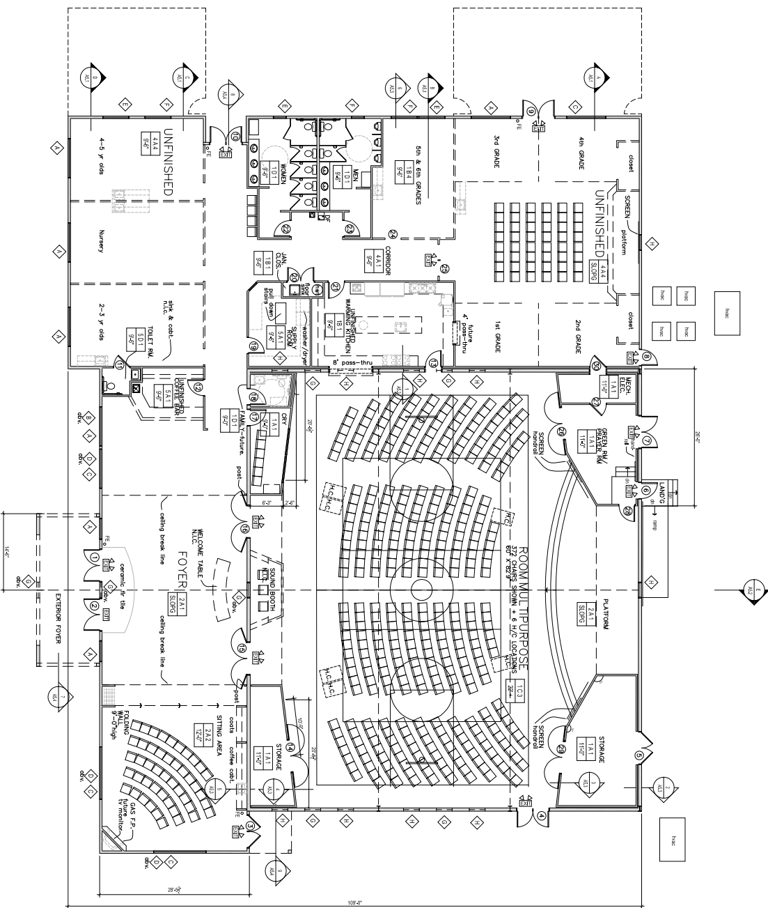
PHASE 1 FLOOR PLAN SCALE: 1/8" = 1'-0" TOTAL SF = 4,378 SF FINISHED TOTAL SF = 4,378 SF UNFINISHED TOTAL SF = 13,848 SF
